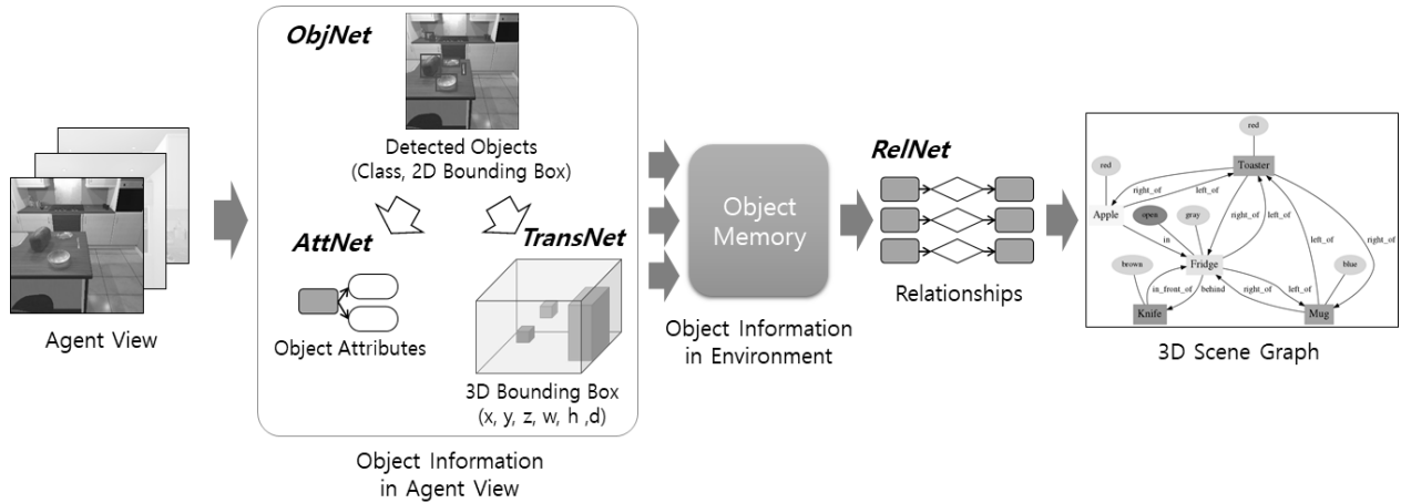
Fig. 3. 3D Scene Graph Generation Model
